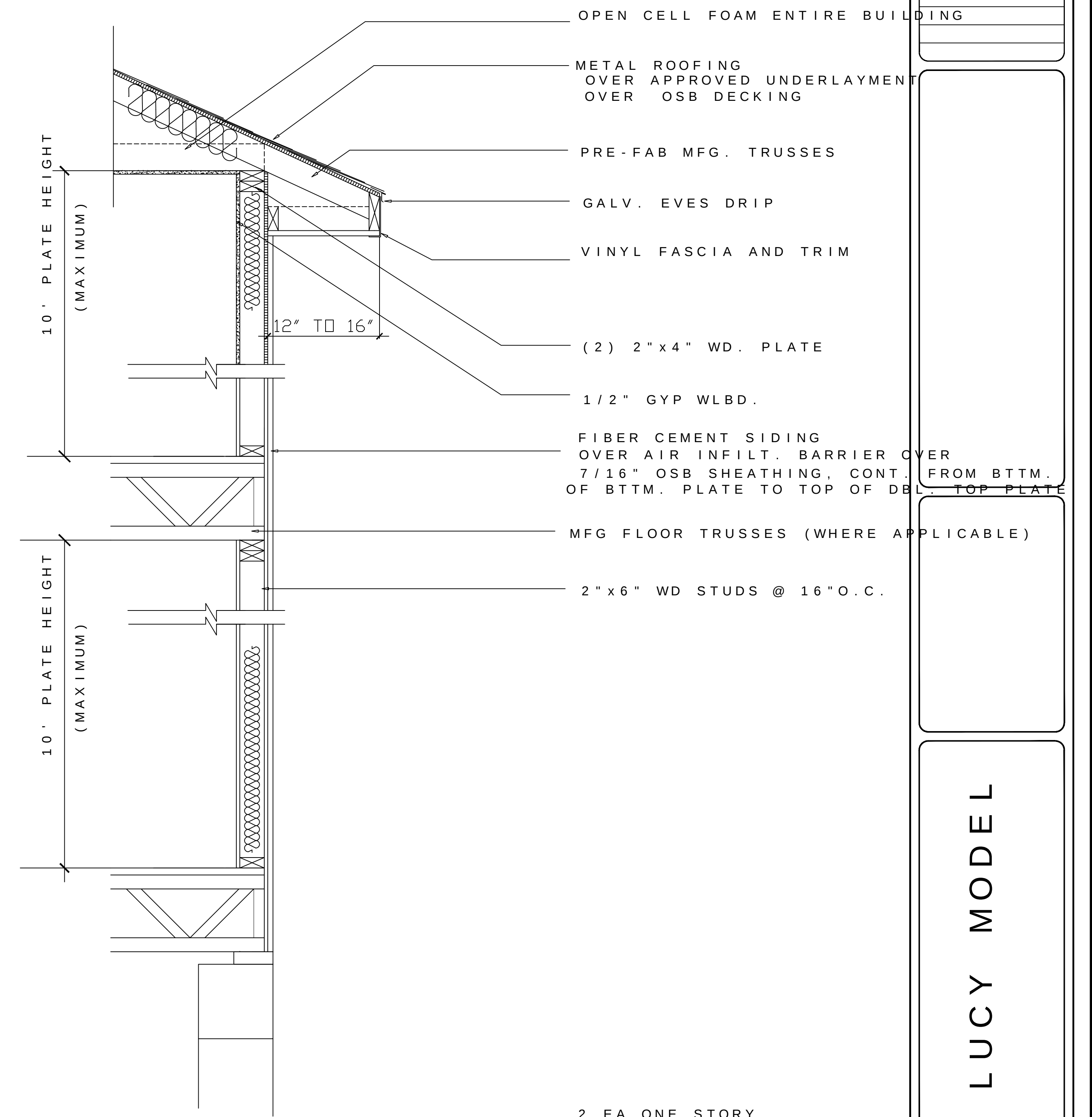
2 EA ONE STORY TYPICAL WALL SECTION A
