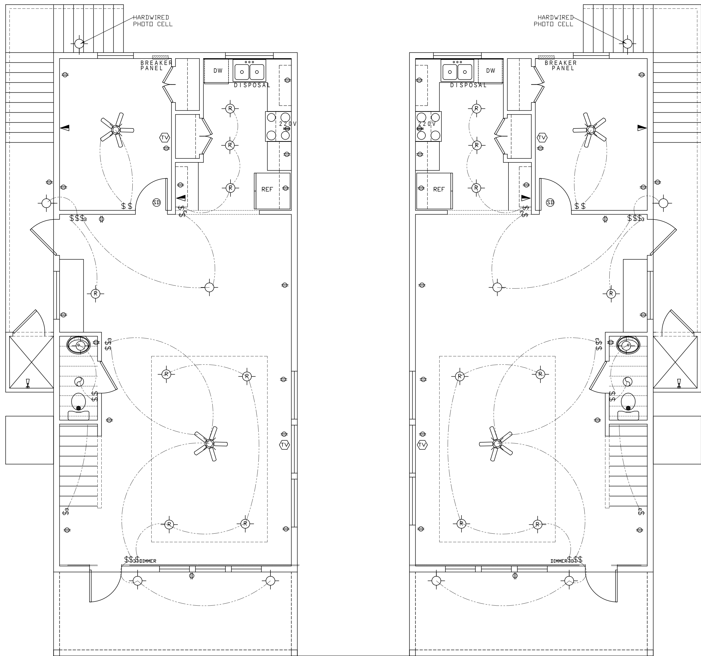
ELECTRICAL PLAN LOWER LEVEL
