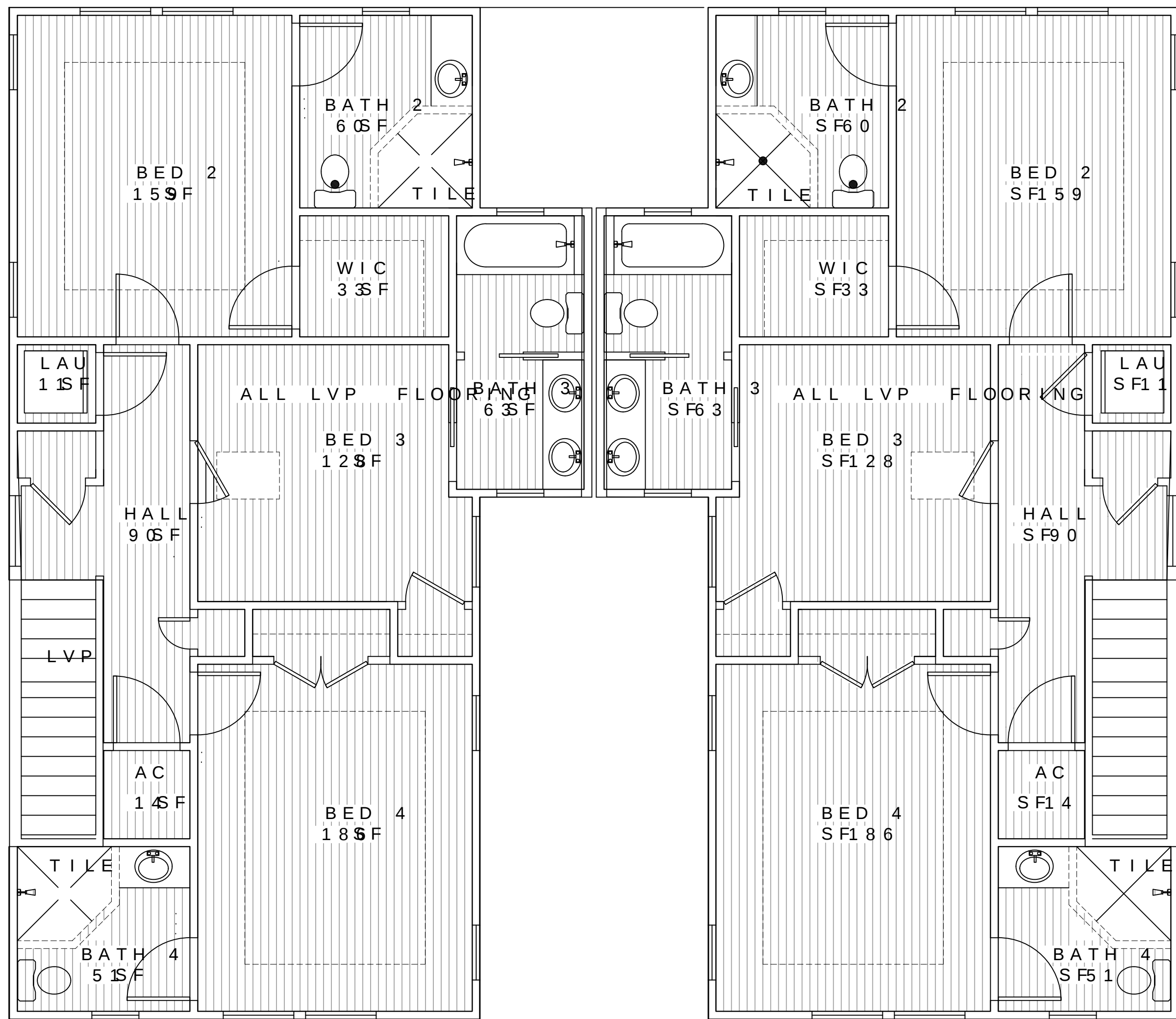
FLOORING PLAN UPPER LEVEL
