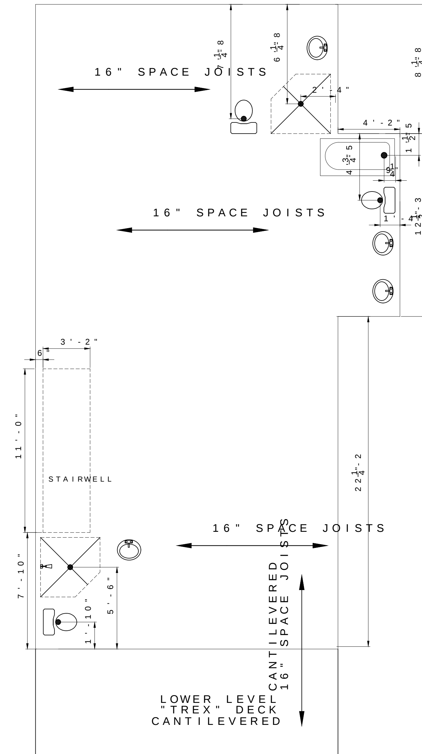
UPPER FLOOR FRAMING SCALE: 1/4"=1'-0"
