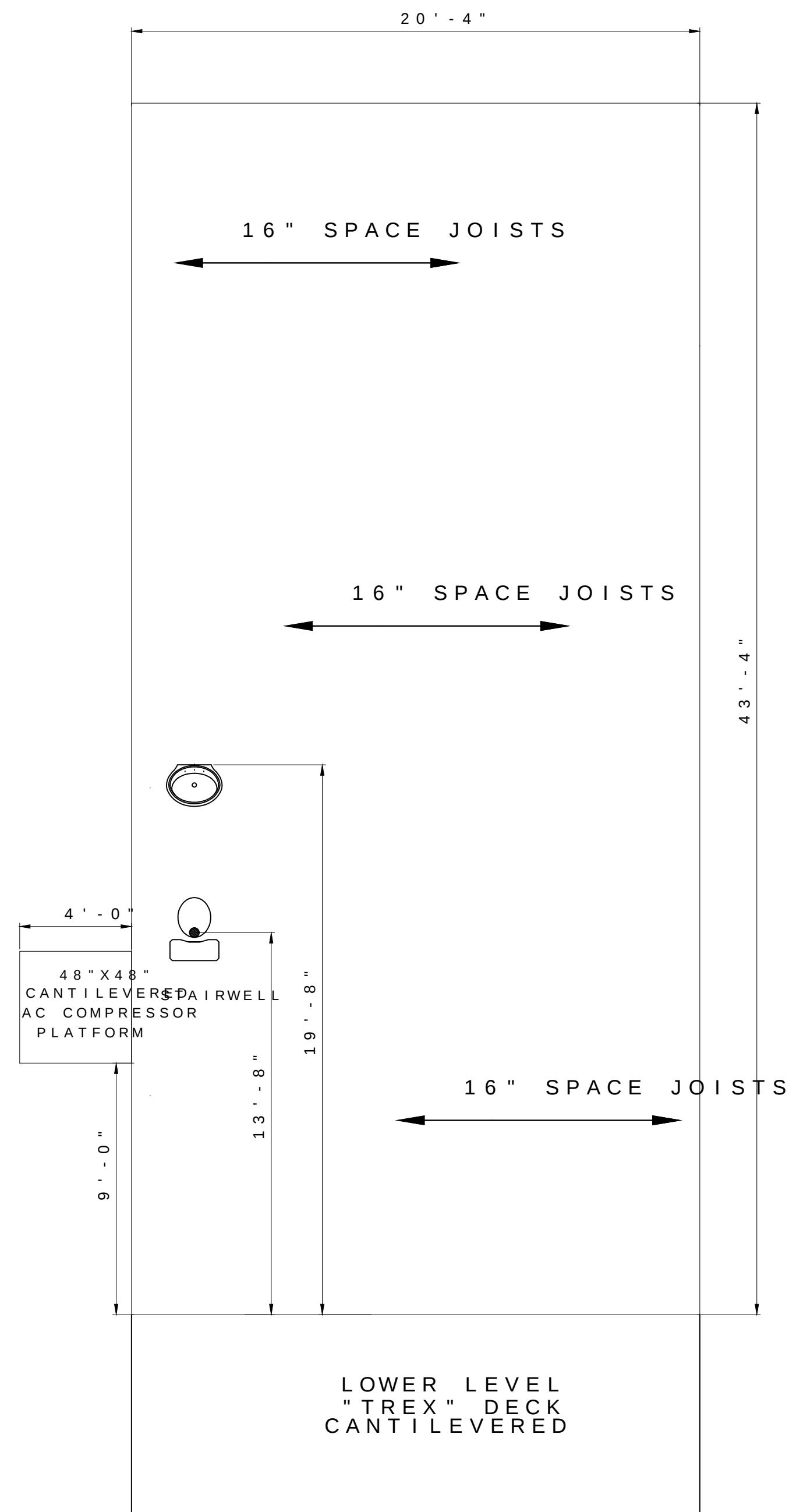
UPPER FLOOR FRAMING SCALE: 1/4"=1'-0"
