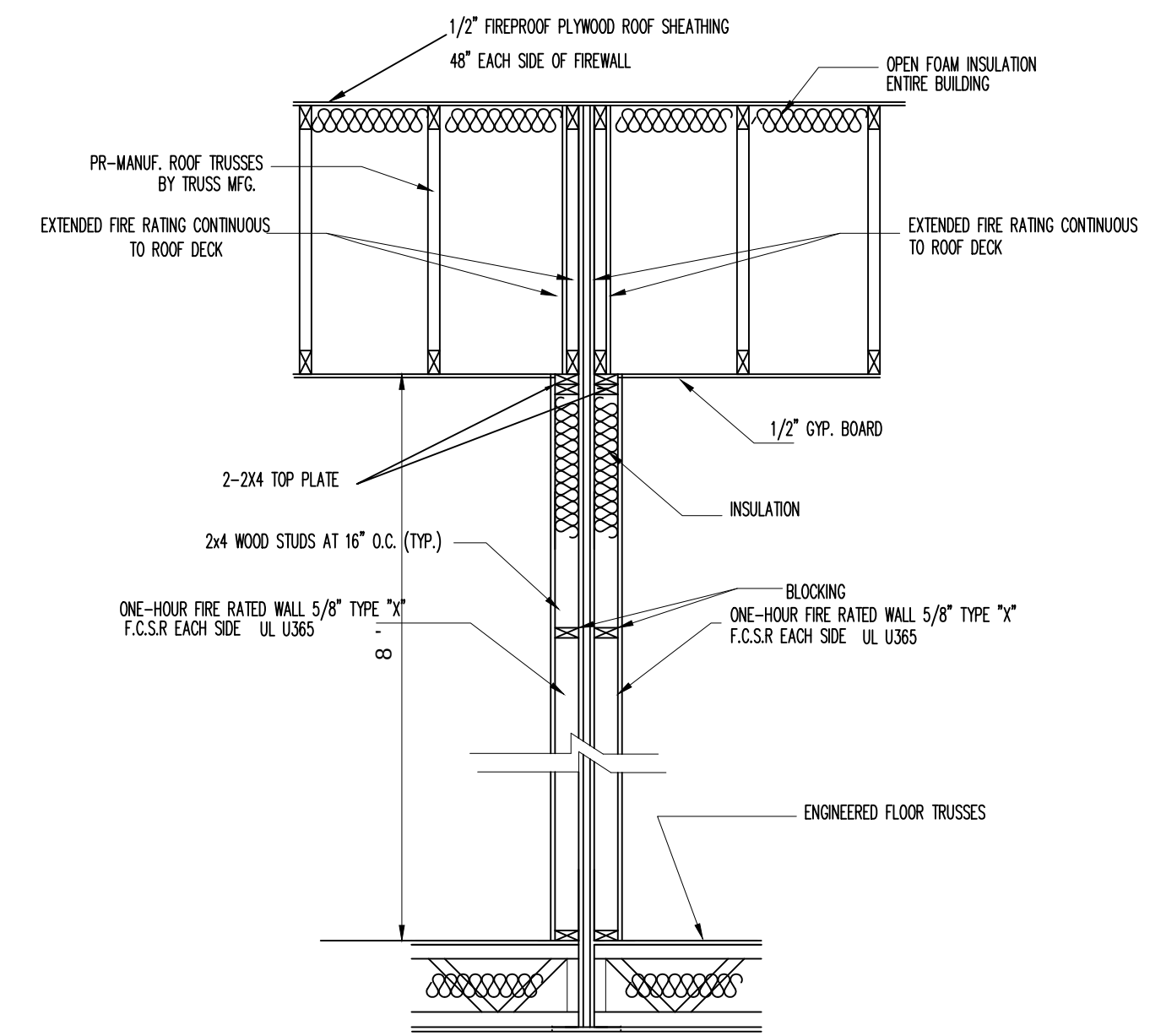
SECTION THRU UPPER LEVEL FIRE WALL SCALE: 1/2" = 1' - 0" SEE ELEVATION FOR SIDING DETAIL
