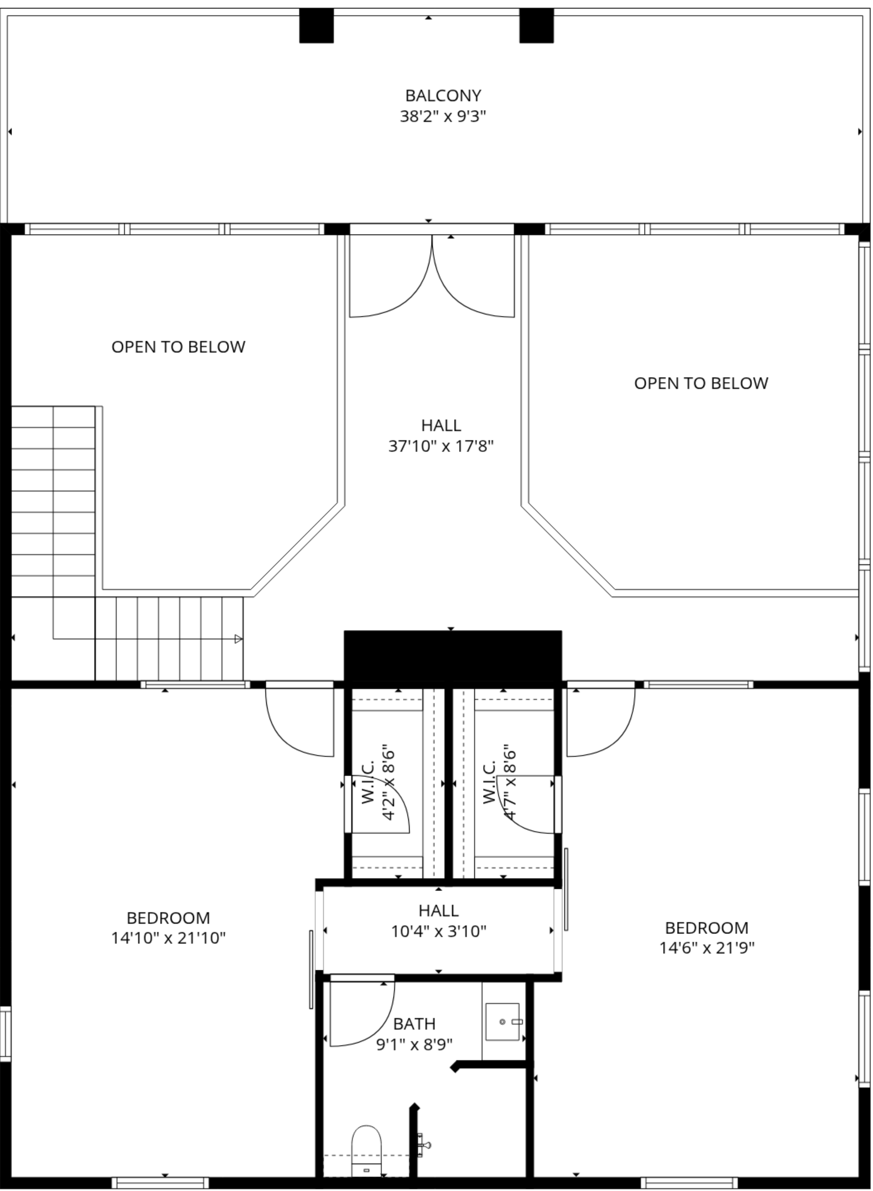
2nd floor
