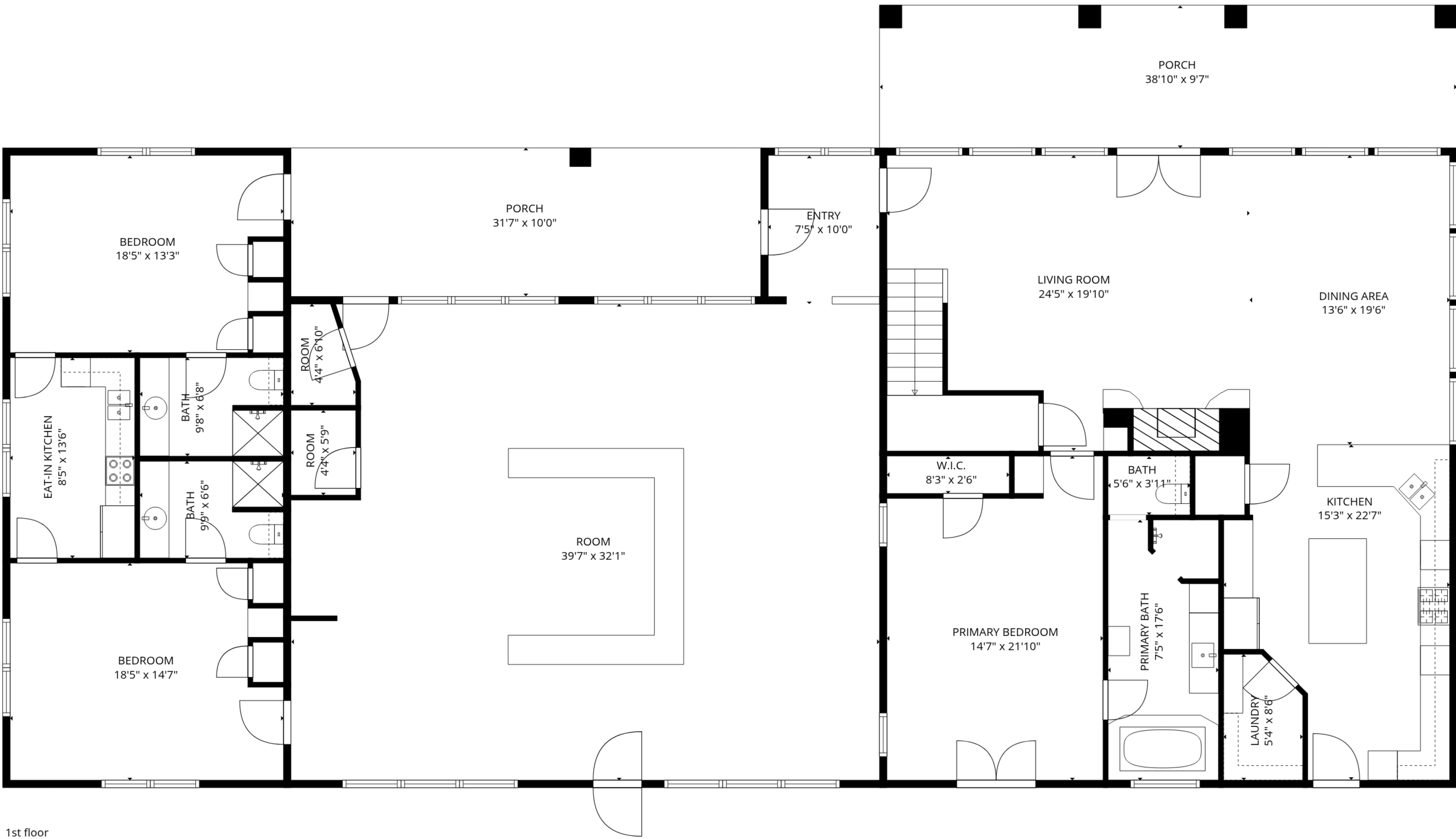
1st floor
